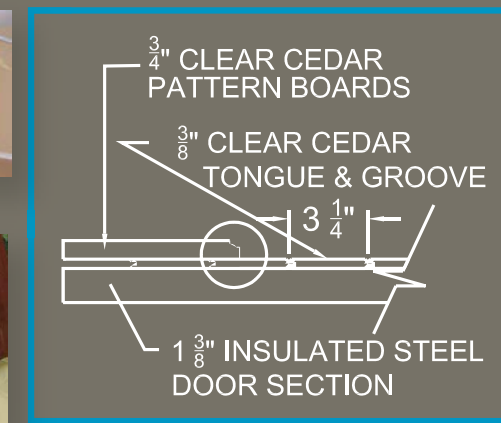
Section Detail
